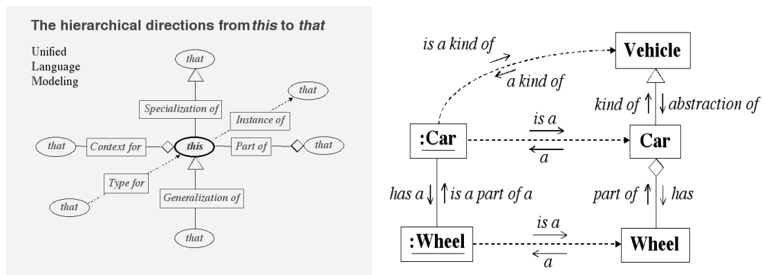
The basic principles of the Unified Language Modeling technique
